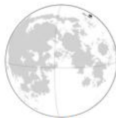
J. Mare Humboldtianum (Humboldt's Sea)
