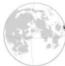
O. Mare Marginis (Border Sea)
