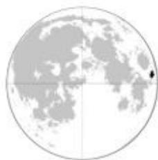
M. Mare Undarum (Sea of Waves)
