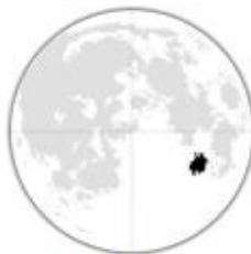
I. Mare Nectaris (Sea of Nectar)
