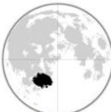
E. Mare Nubium (Sea of Clouds)
