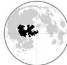
D. Mare Insularum (Sea of Isles)
